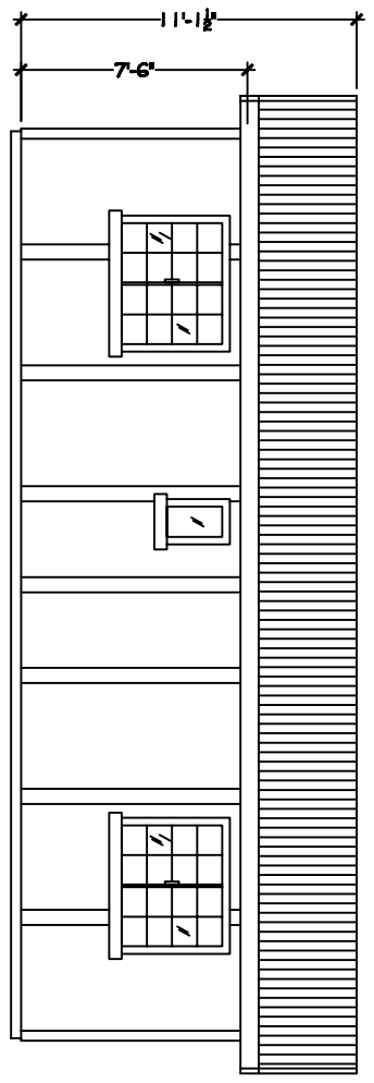
3 REAR ELEVATION SCALE: 1/4" = 1'-0"
